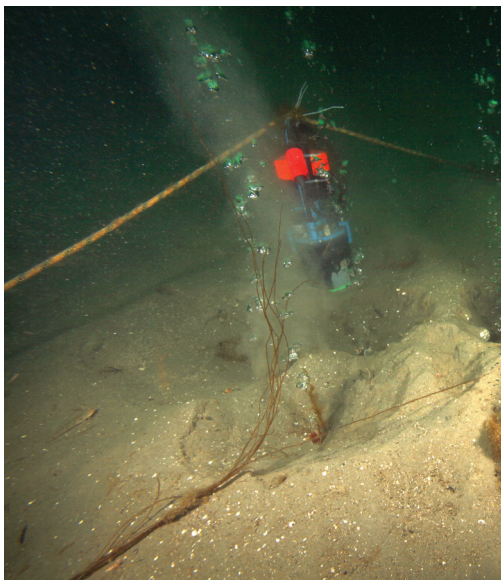
Fig 1: SeaGuard deployed in QICS project at epicenter during a period of CO 2 release. Bubbles were normally only visible during low tide. They dissolve as they rise and are never visible at the surface. Photo courtesy of Henrik Stahl, Zayed University, UAE.
